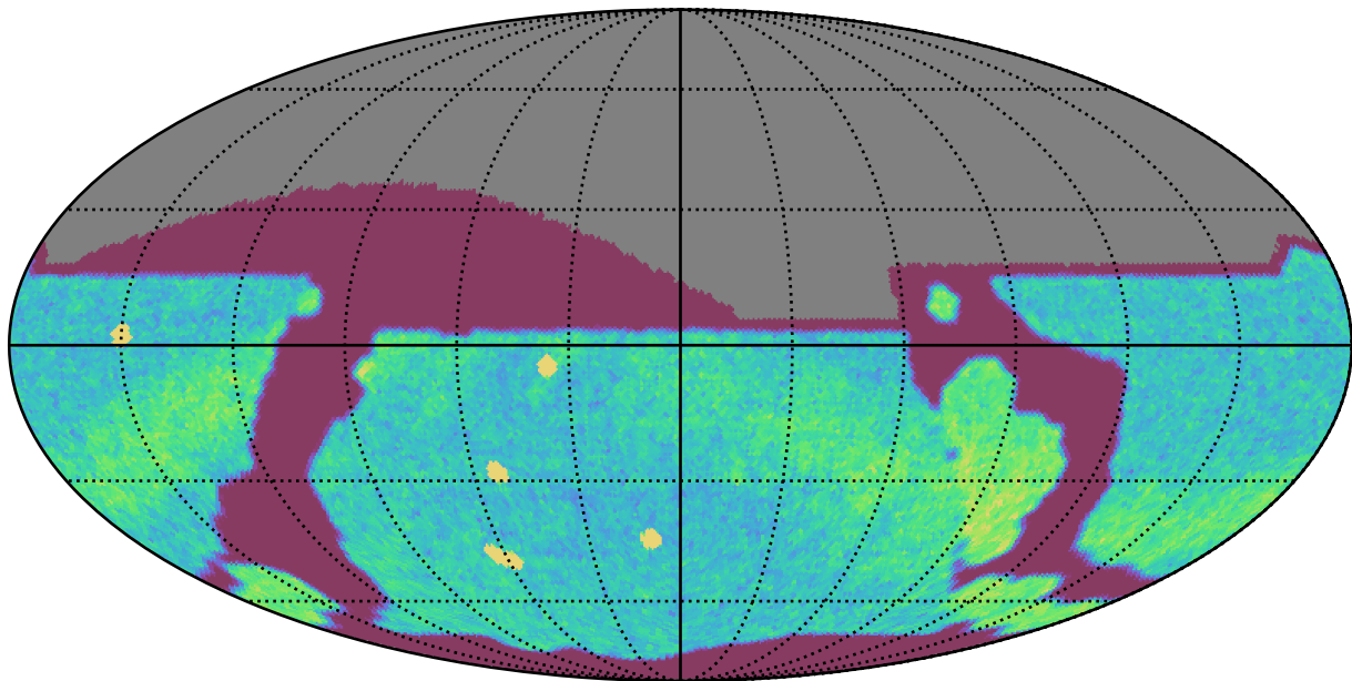
too_elab_r8_d2_giz_v3.4_10yrs All sky r band: NVisits
