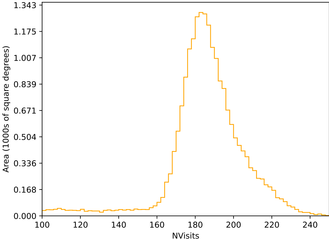
too_elab_r8_d2_giz_v3.4_10yrs All sky r band: NVisits
