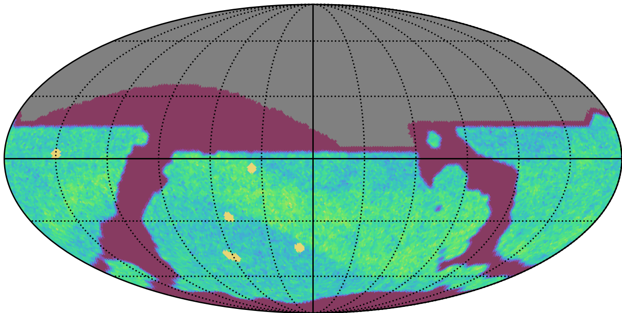
too_elab_r8_d2_giz_v3.4_10yrs All sky i band: NVisits
