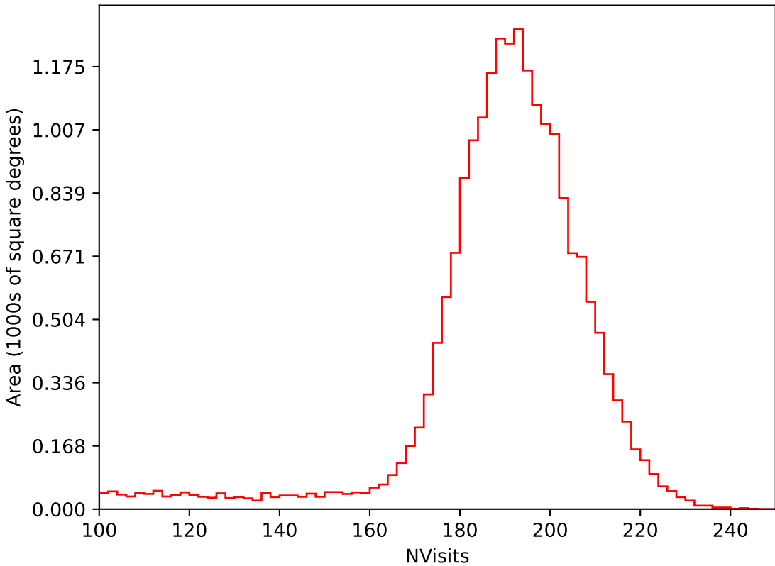
too_elab_r8_d2_giz_v3.4_10yrs All sky i band: NVisits
