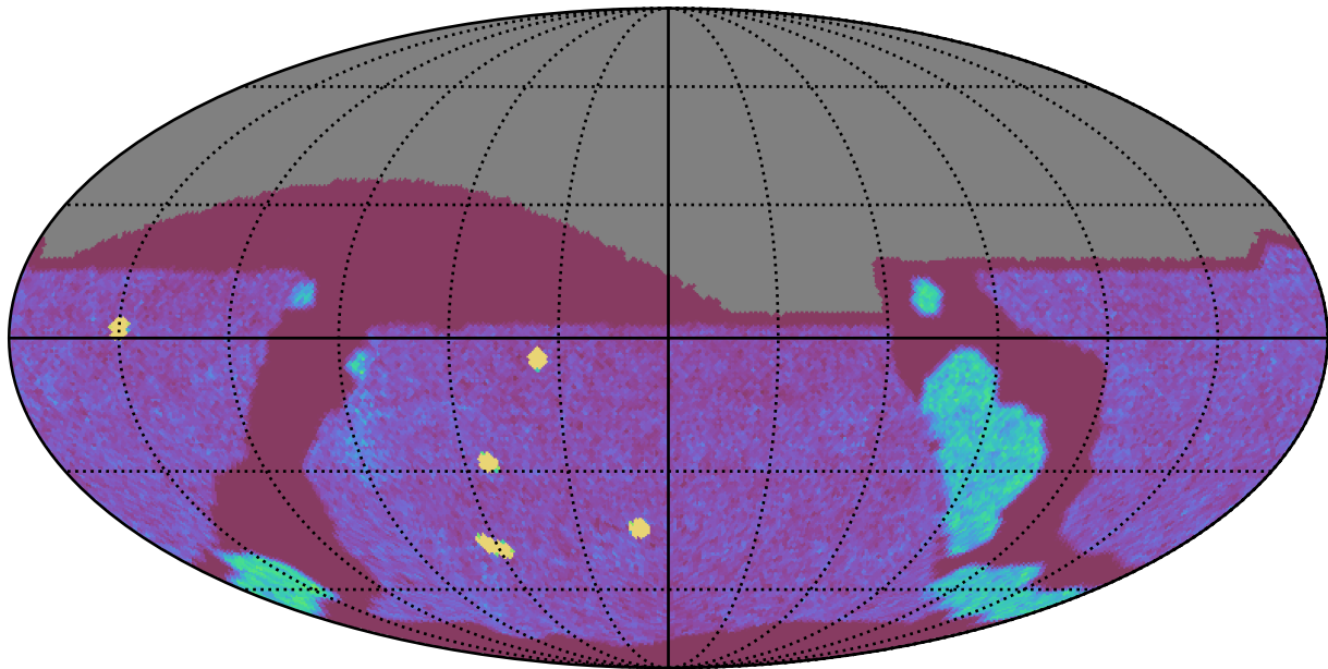
too_elab_r8_d2_giz_v3.4_10yrs All sky g band: NVisits
