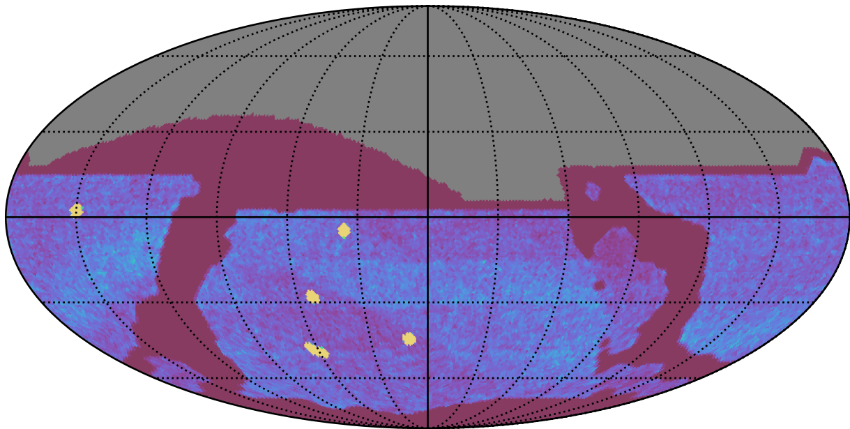
too_elab_r8_d2_giz_v3.4_10yrs All sky all bands: NVisits
