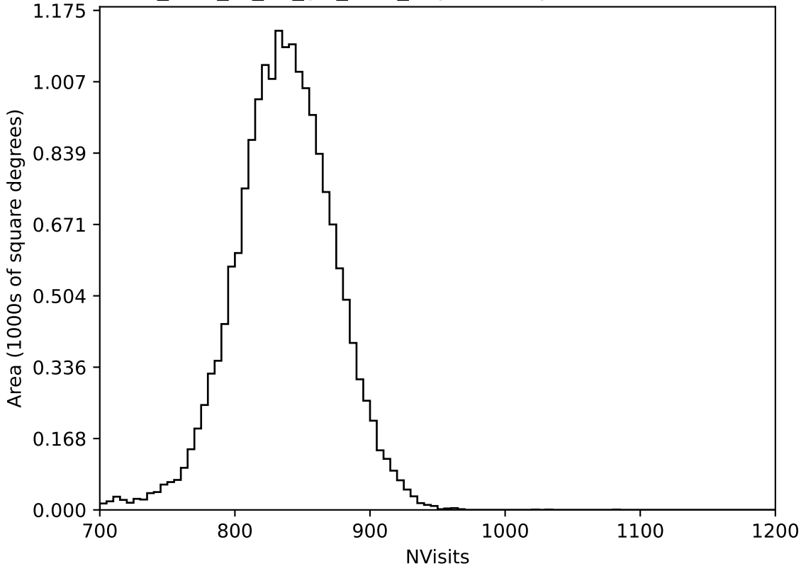
too_elab_r8_d2_giz_v3.4_10yrs All sky all bands: NVisits
