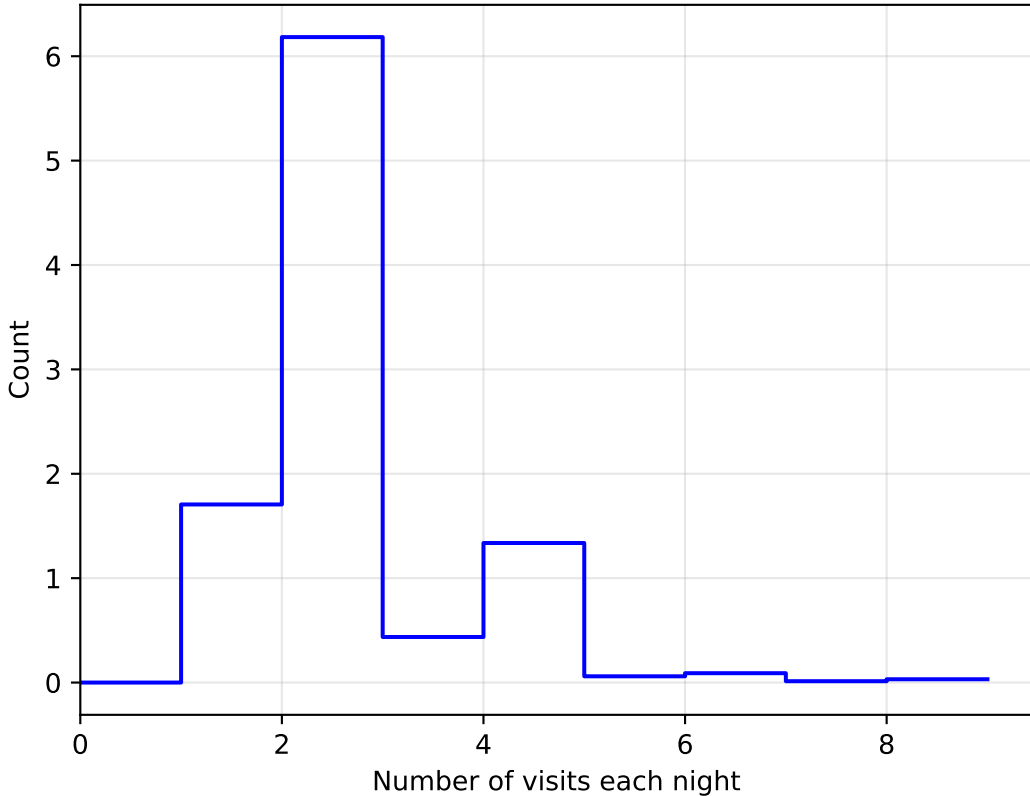
too_elab_r8_d2_giz_v3.4_10yrs All sky: NVisitsPerNight
