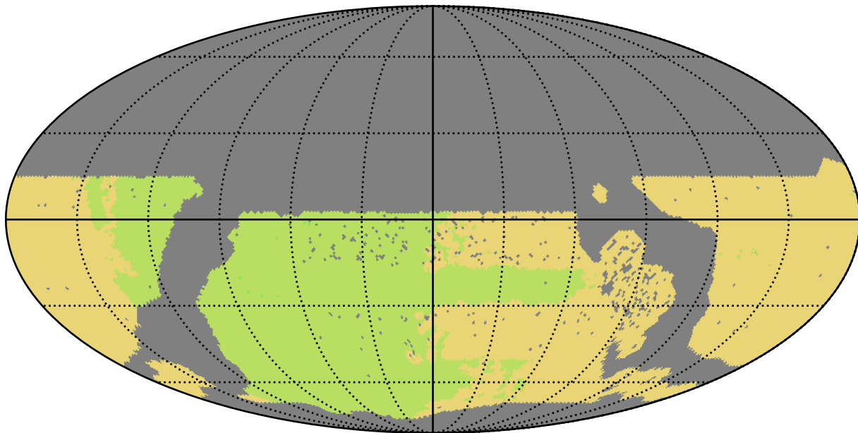
too_elab_r8_d2_giz_v3.4_10yrs WFD all bands: NSeasons
