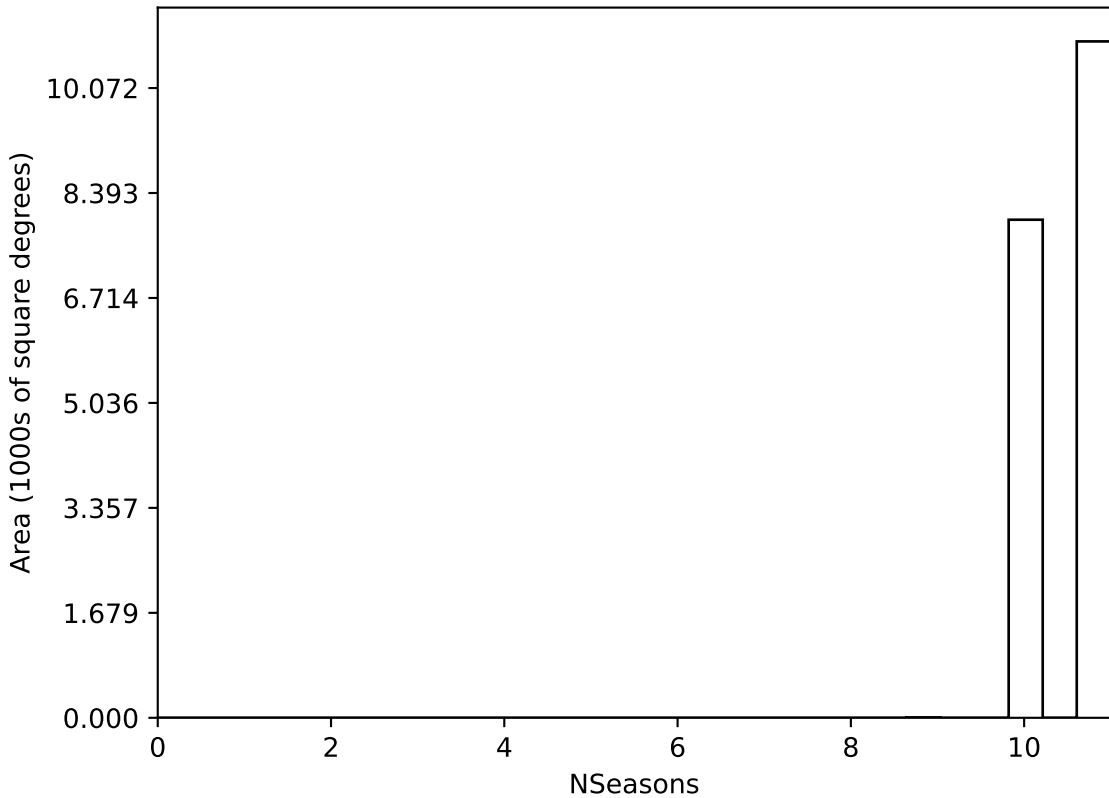
too_elab_r8_d2_giz_v3.4_10yrs WFD all bands: NSeasons
