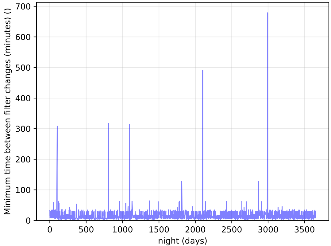
too_elab_r8_d2_giz_v3.4_10yrs Per Night: Minimum time between filter changes (minutes)
