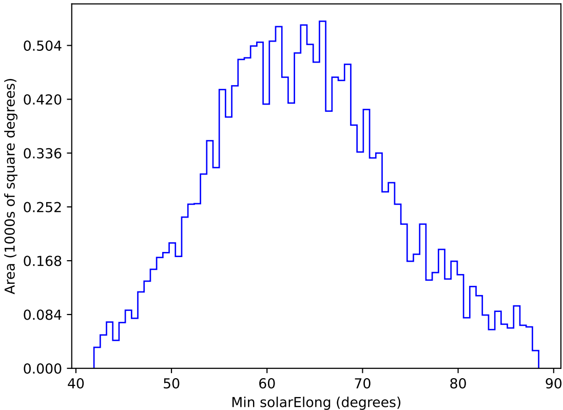
too_elab_r8_d2_giz_v3.4_10yrs WFD y band: Min solarElong
