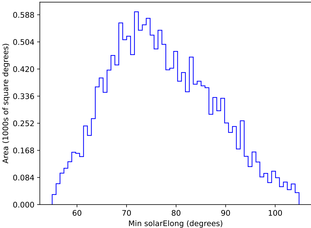
too_elab_r8_d2_giz_v3.4_10yrs WFD u band: Min solarElong
