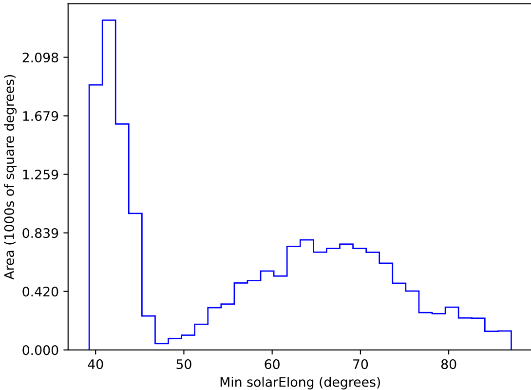
too_elab_r8_d2_giz_v3.4_10yrs WFD r band: Min solarElong
