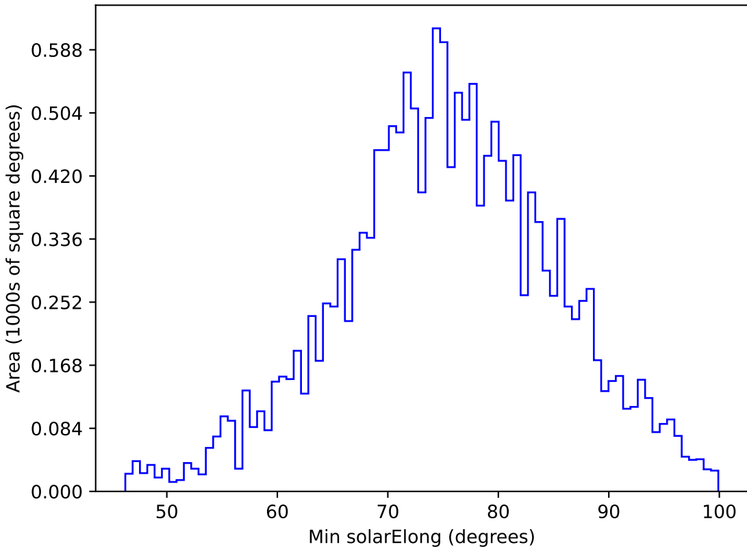
too_elab_r8_d2_giz_v3.4_10yrs WFD g band: Min solarElong
