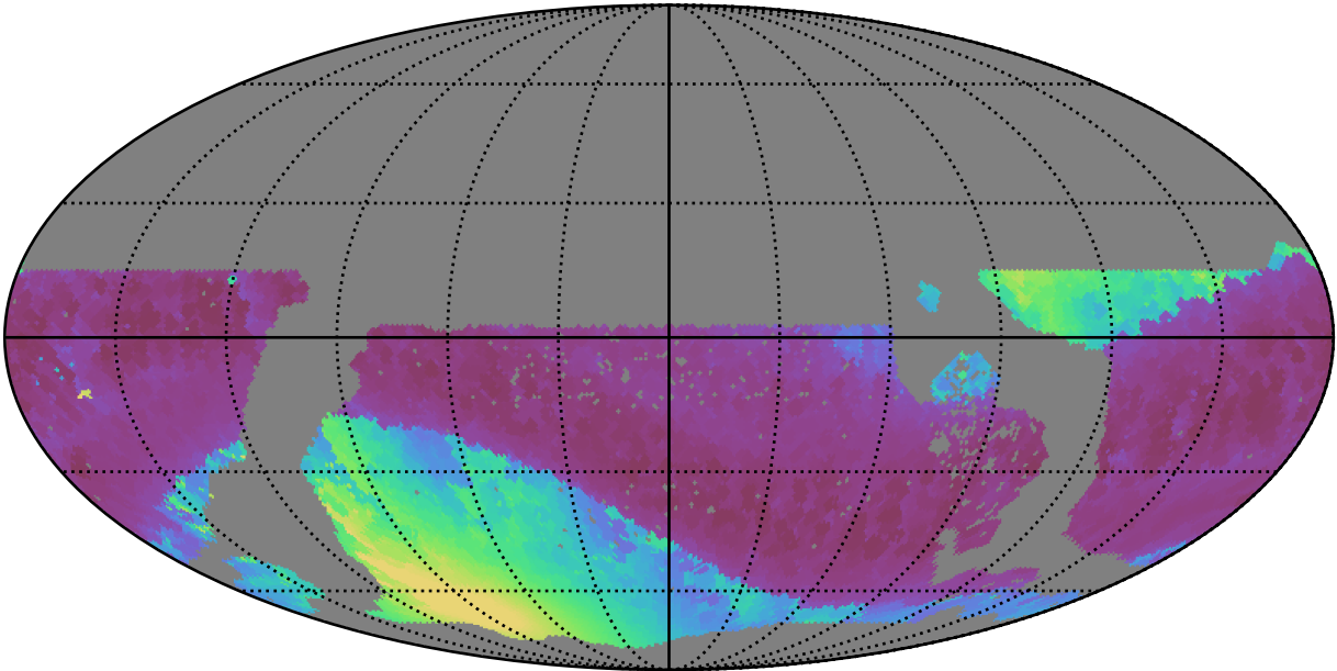
too_elab_r8_d2_giz_v3.4_10yrs WFD all bands: Min solarElong
