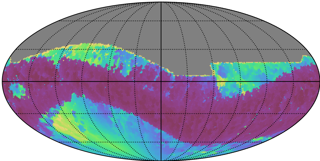
too_elab_r8_d2_giz_v3.4_10yrs All sky z band: Min solarElong
