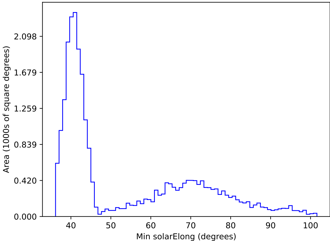
too_elab_r8_d2_giz_v3.4_10yrs All sky z band: Min solarElong
