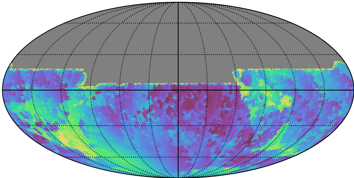
too_elab_r8_d2_giz_v3.4_10yrs All sky y band: Min solarElong
