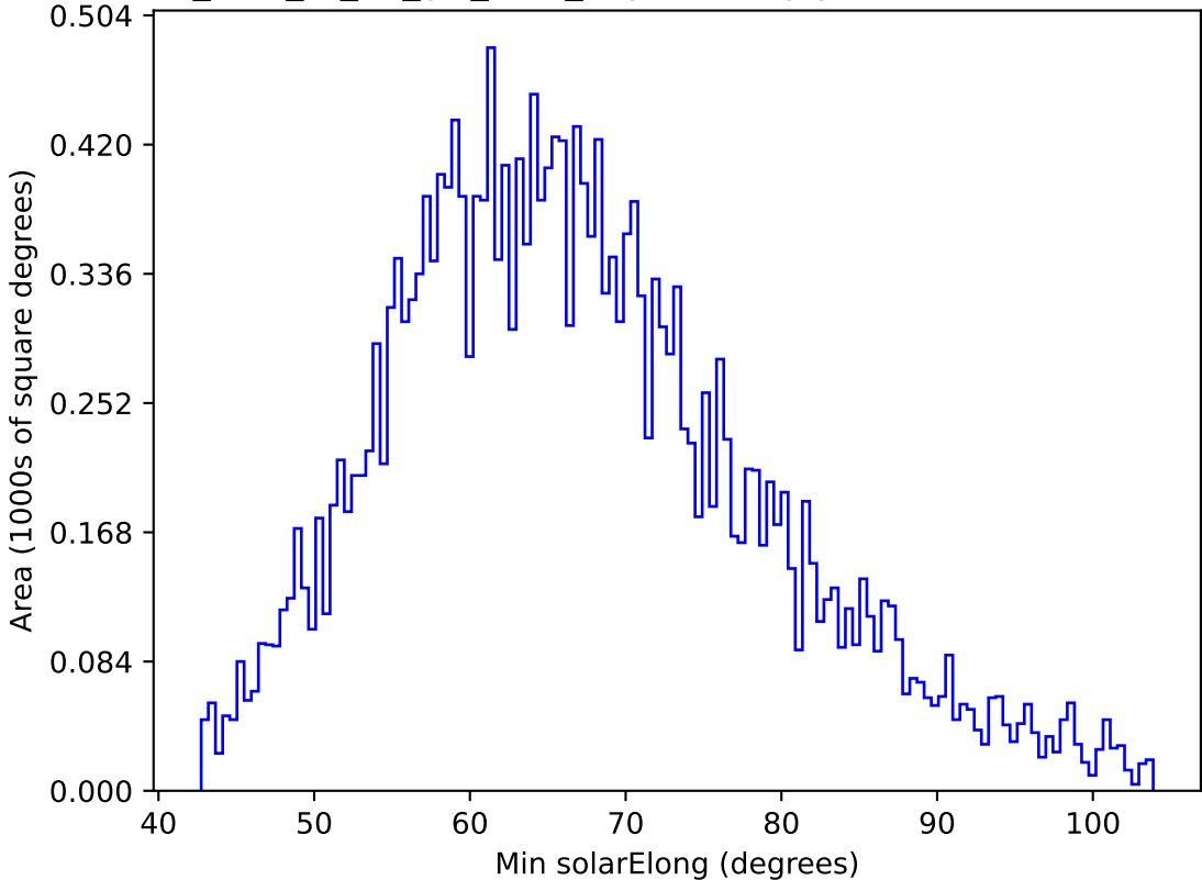
too_elab_r8_d2_giz_v3.4_10yrs All sky y band: Min solarElong
