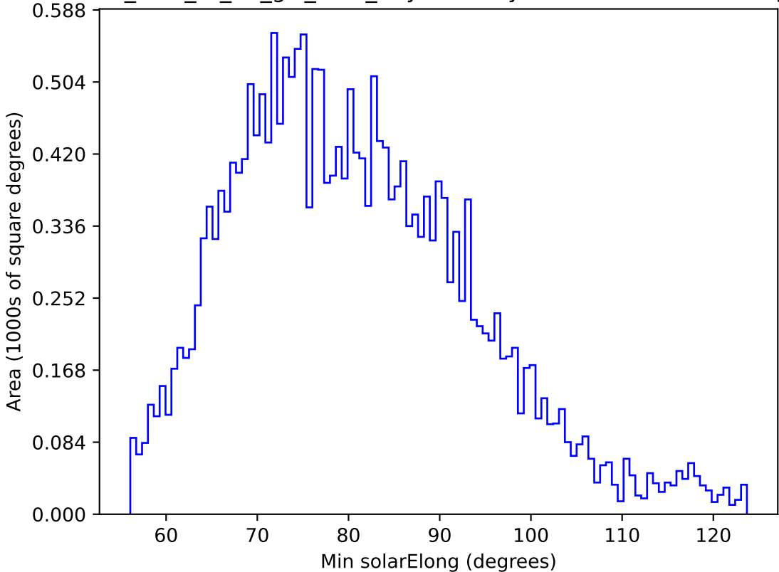
too_elab_r8_d2_giz_v3.4_10yrs All sky u band: Min solarElong
