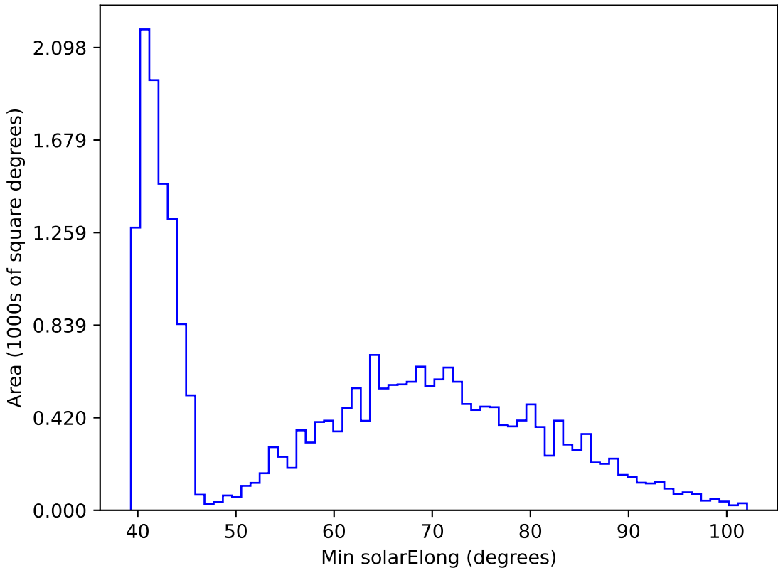
too_elab_r8_d2_giz_v3.4_10yrs All sky r band: Min solarElong
