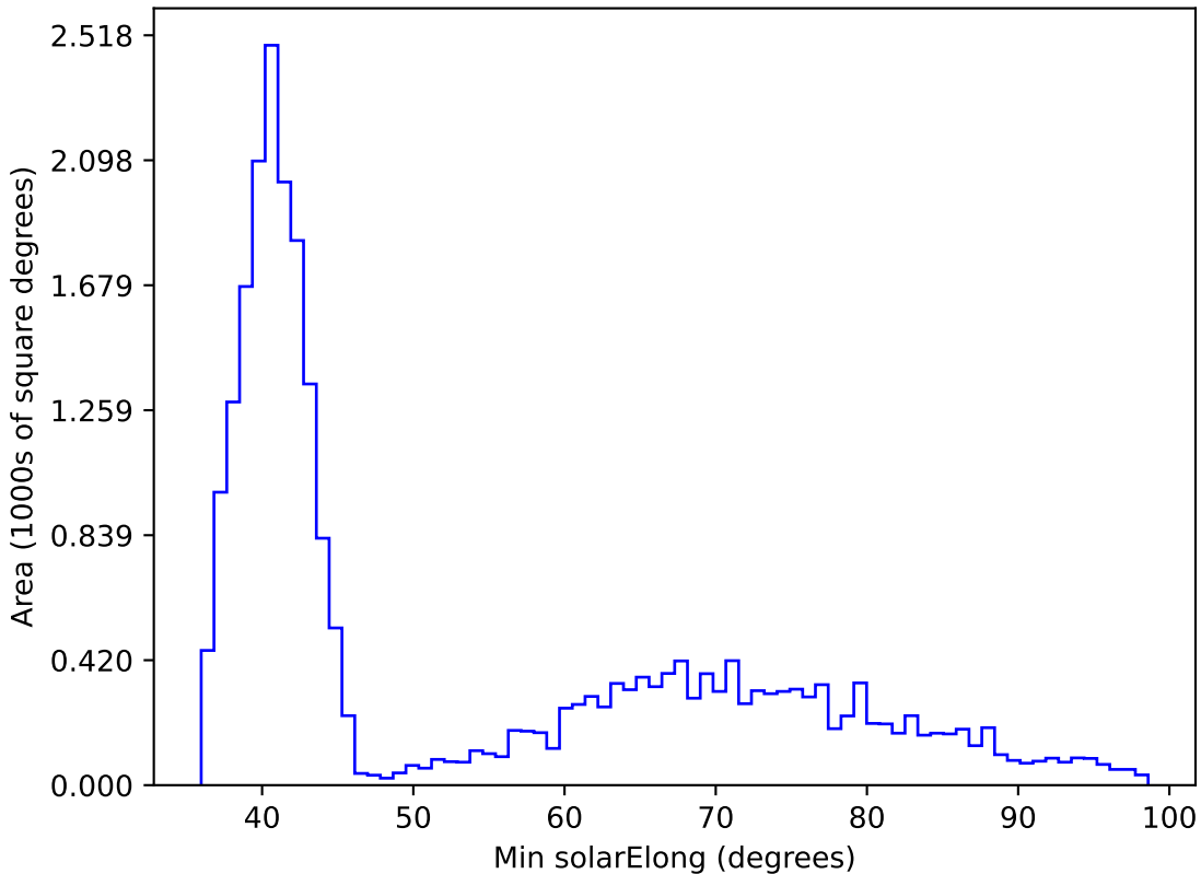
too_elab_r8_d2_giz_v3.4_10yrs All sky i band: Min solarElong
