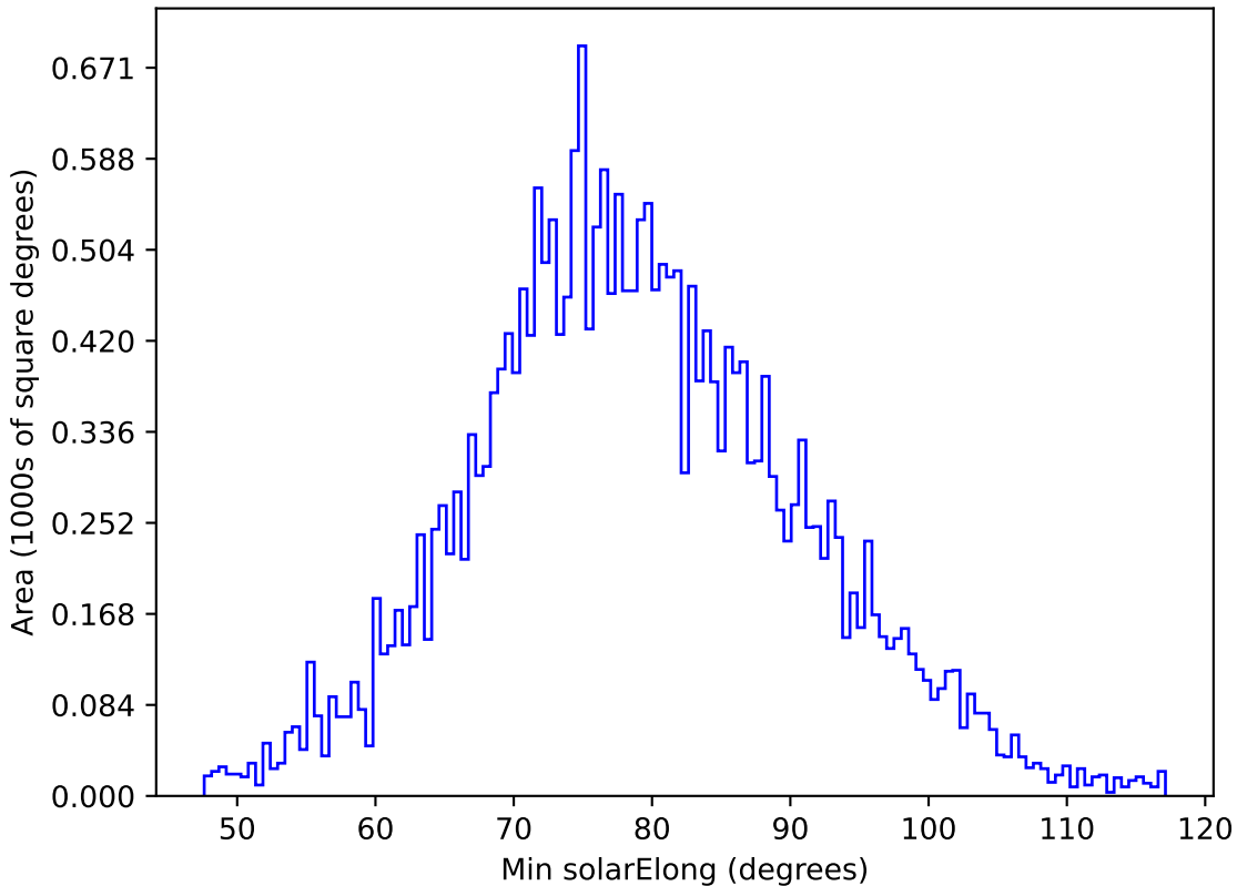
too_elab_r8_d2_giz_v3.4_10yrs All sky g band: Min solarElong
