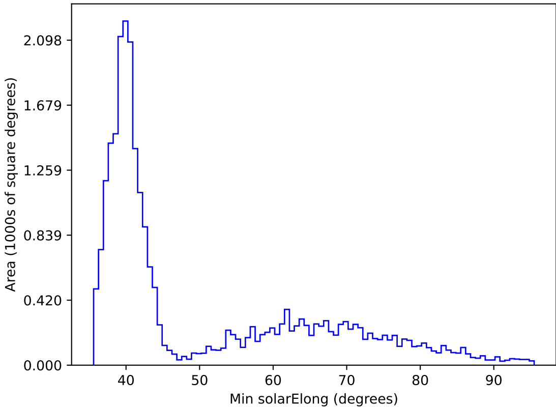
too_elab_r8_d2_giz_v3.4_10yrs All sky all bands: Min solarElong
