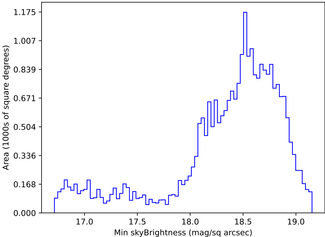
too_elab_r8_d2_giz_v3.4_10yrs Yr 1 z band: Min skyBrightness
