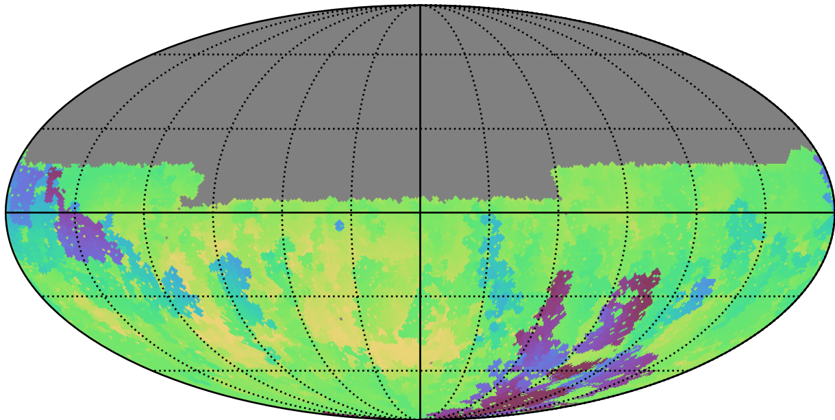
too_elab_r8_d2_giz_v3.4_10yrs Yr 1 u band: Min skyBrightness
