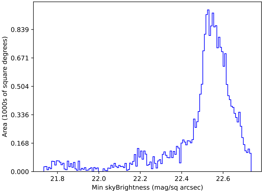
too_elab_r8_d2_giz_v3.4_10yrs Yr 1 u band: Min skyBrightness
