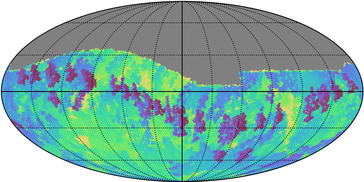
too_elab_r8_d2_giz_v3.4_10yrs Yr 1 i band: Min skyBrightness
