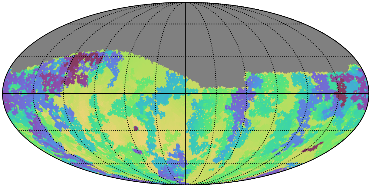
too_elab_r8_d2_giz_v3.4_10yrs Yr 1 g band: Min skyBrightness
