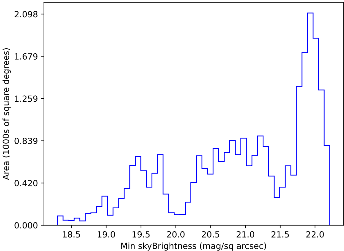
too_elab_r8_d2_giz_v3.4_10yrs Yr 1 g band: Min skyBrightness
