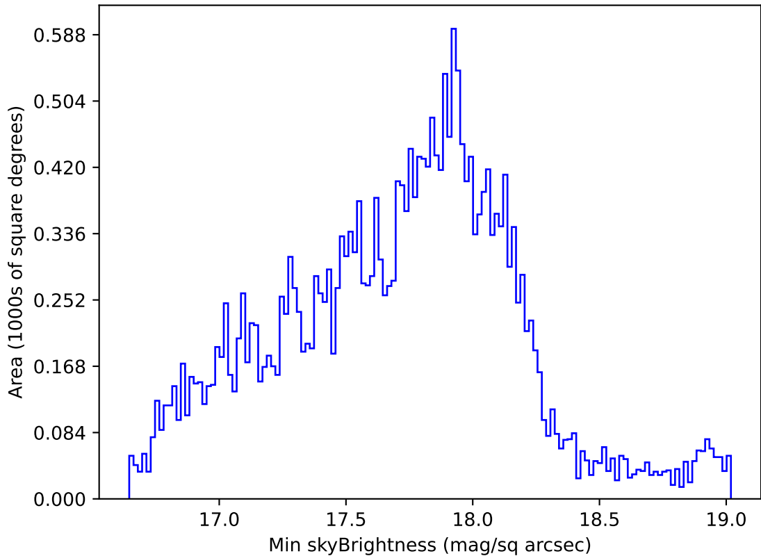
too_elab_r8_d2_giz_v3.4_10yrs Yr 1 all bands: Min skyBrightness
