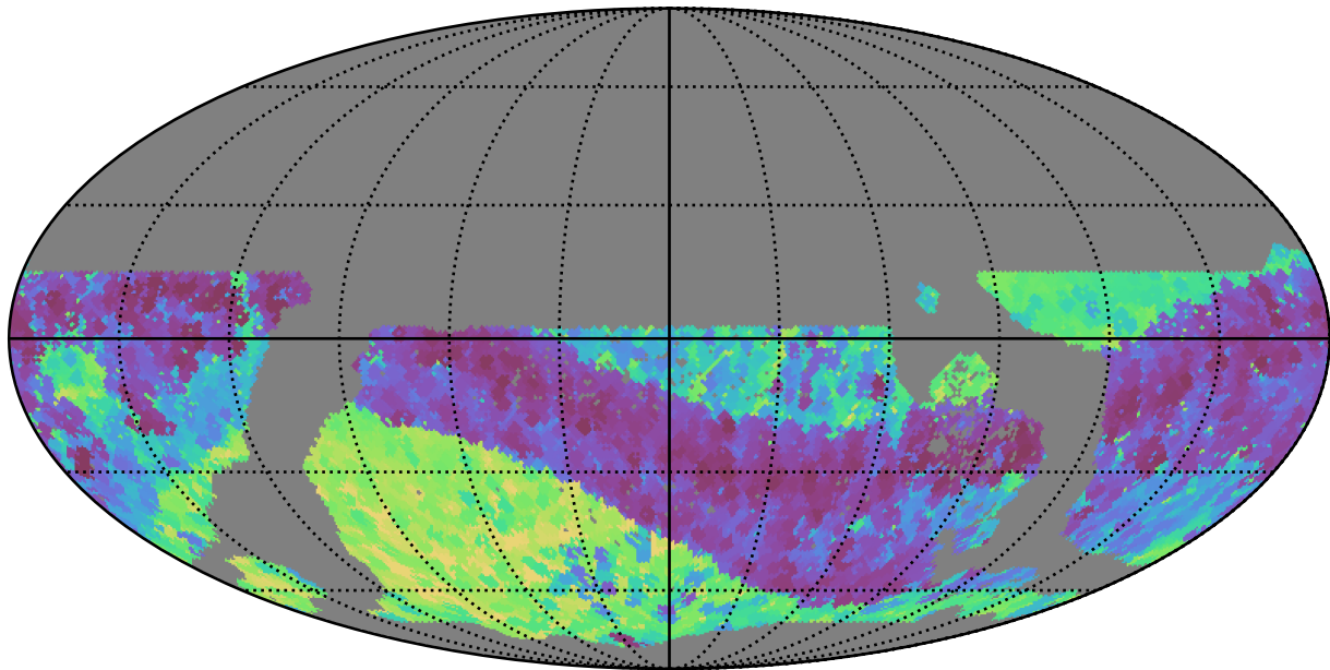
too_elab_r8_d2_giz_v3.4_10yrs WFD z band: Min skyBrightness
