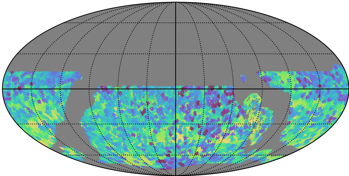
too_elab_r8_d2_giz_v3.4_10yrs WFD y band: Min skyBrightness
