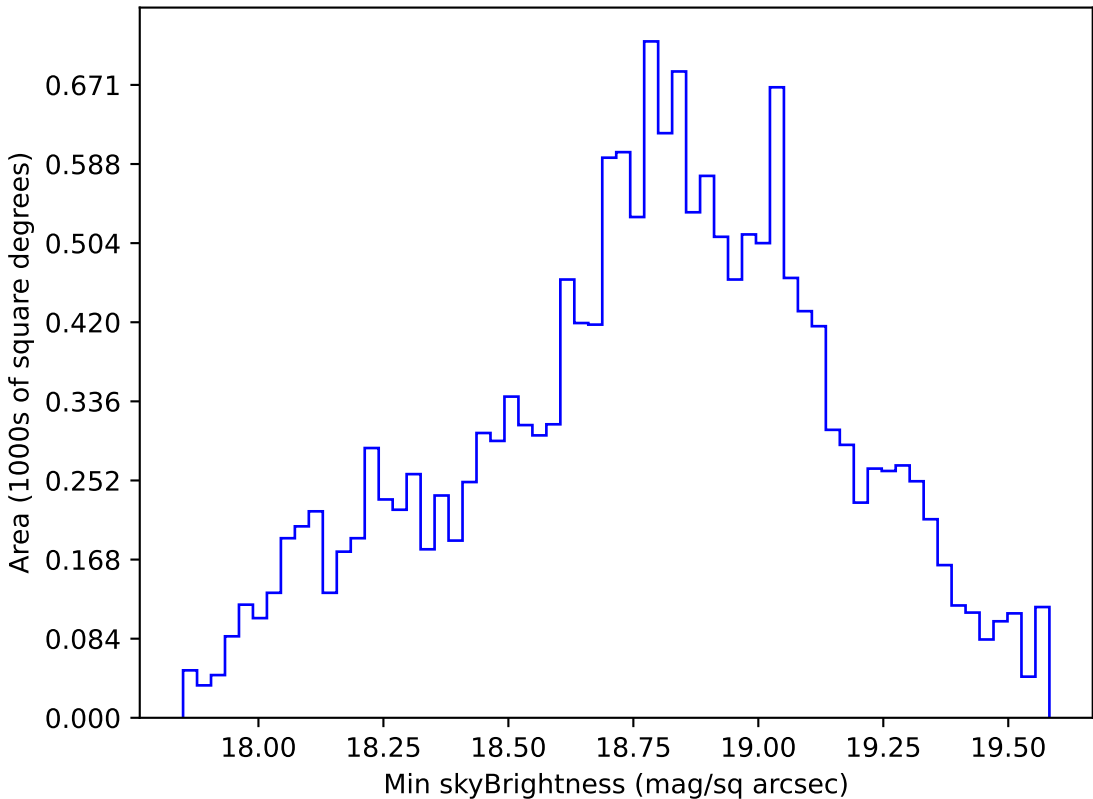
too_elab_r8_d2_giz_v3.4_10yrs WFD r band: Min skyBrightness
