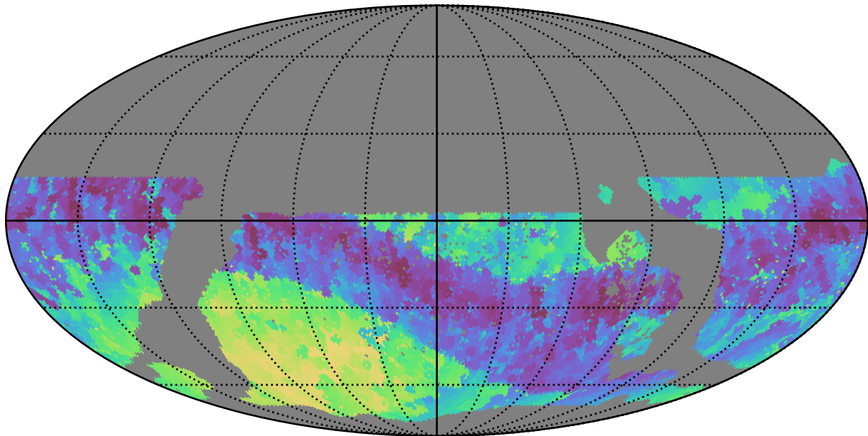
too_elab_r8_d2_giz_v3.4_10yrs WFD i band: Min skyBrightness
