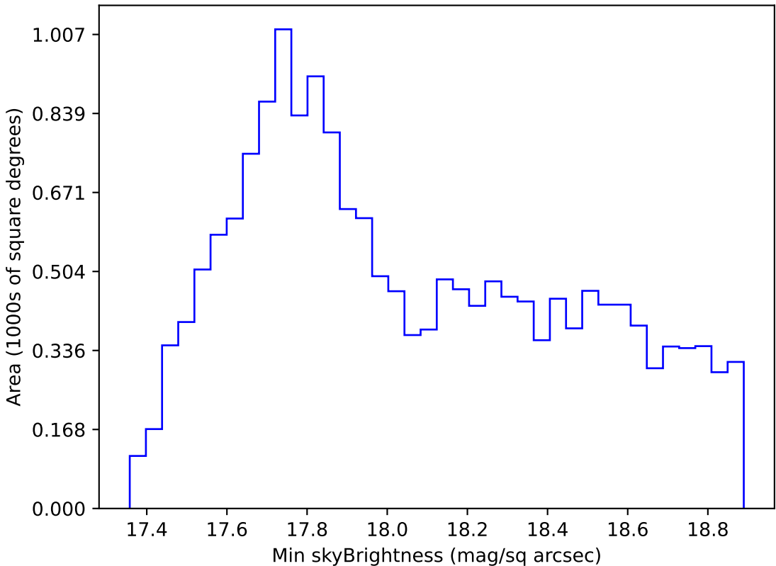
too_elab_r8_d2_giz_v3.4_10yrs WFD i band: Min skyBrightness
