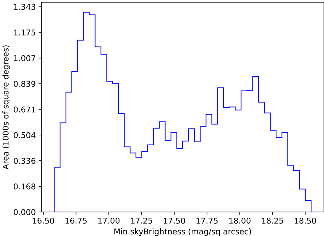
too_elab_r8_d2_giz_v3.4_10yrs All sky z band: Min skyBrightness
