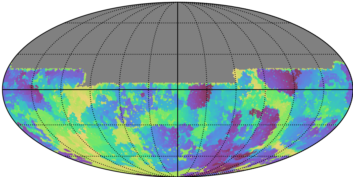
too_elab_r8_d2_giz_v3.4_10yrs All sky u band: Min skyBrightness
