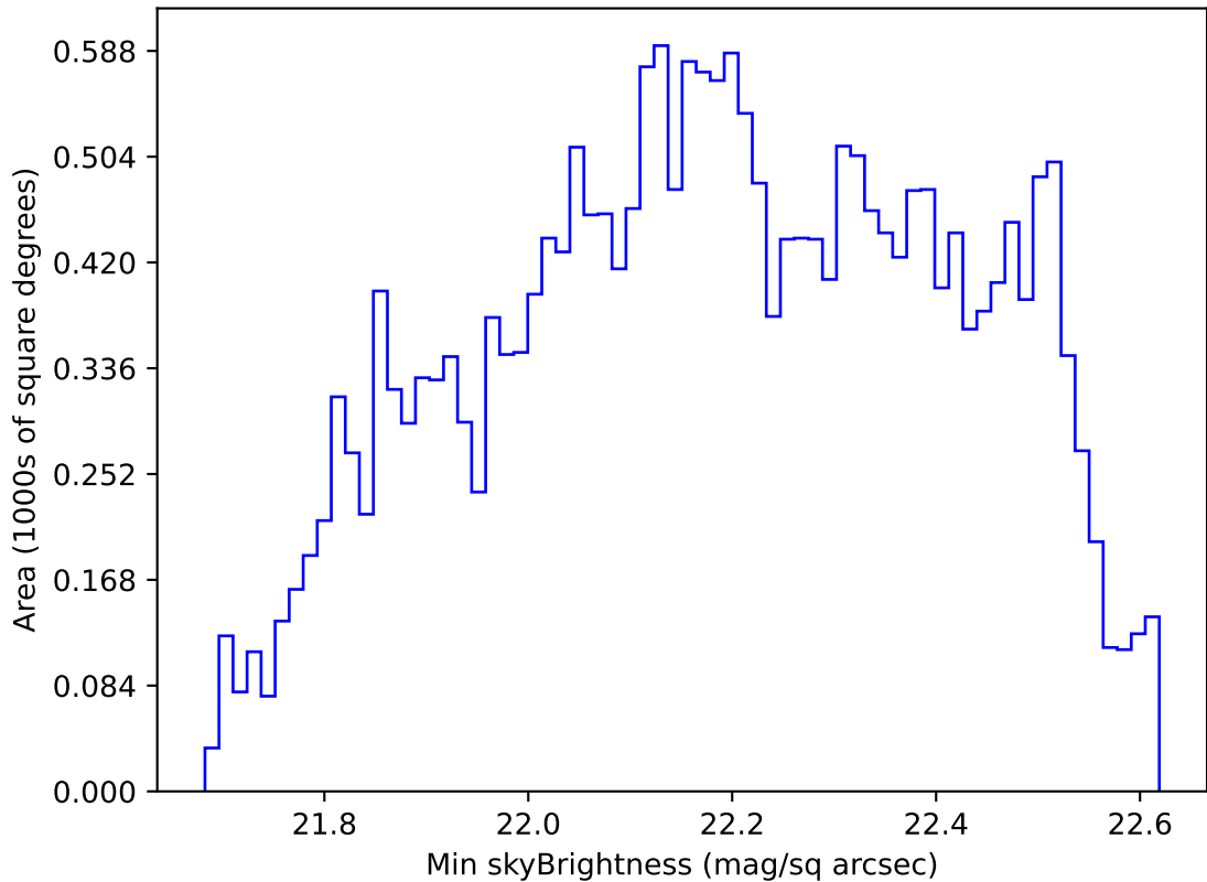
too_elab_r8_d2_giz_v3.4_10yrs All sky u band: Min skyBrightness
