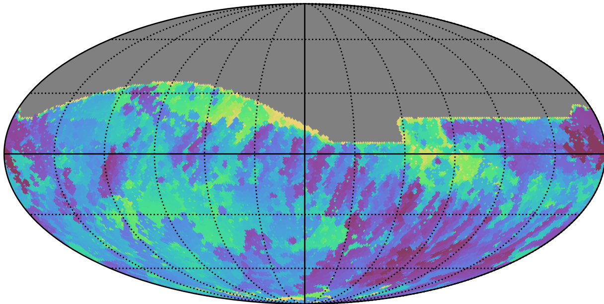
too_elab_r8_d2_giz_v3.4_10yrs All sky r band: Min skyBrightness
