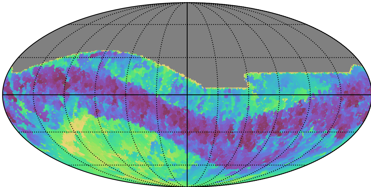
too_elab_r8_d2_giz_v3.4_10yrs All sky i band: Min skyBrightness
