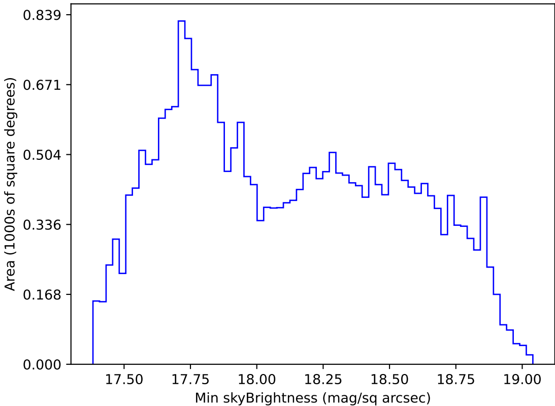
too_elab_r8_d2_giz_v3.4_10yrs All sky i band: Min skyBrightness
