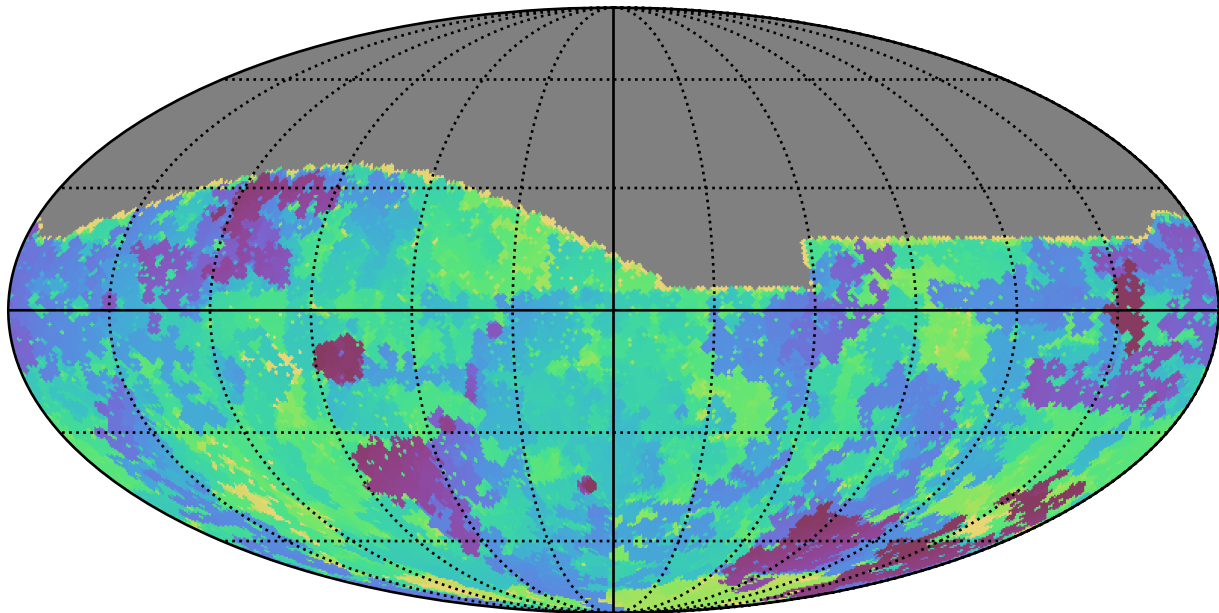
too_elab_r8_d2_giz_v3.4_10yrs All sky g band: Min skyBrightness
