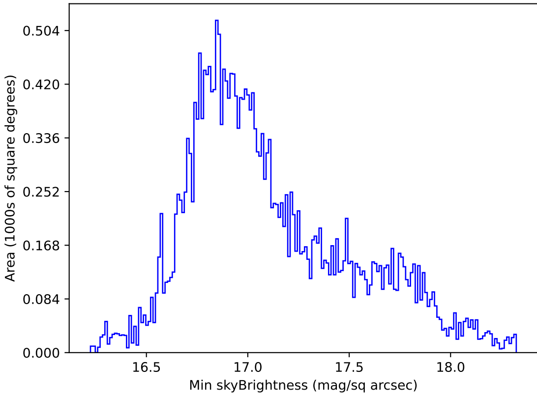
too_elab_r8_d2_giz_v3.4_10yrs All sky all bands: Min skyBrightness
