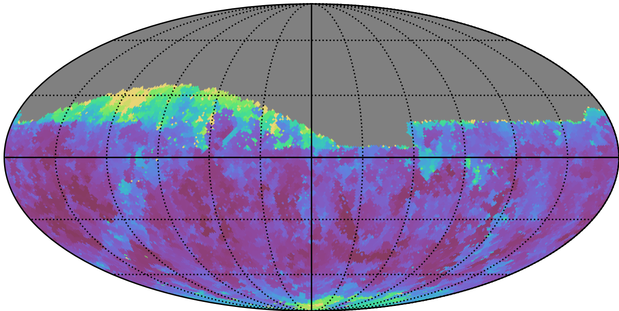
too_elab_r8_d2_giz_v3.4_10yrs Yr 1 z band: Min seeingGeom
