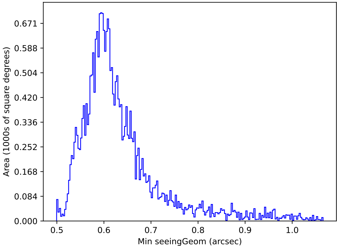
too_elab_r8_d2_giz_v3.4_10yrs Yr 1 i band: Min seeingGeom
