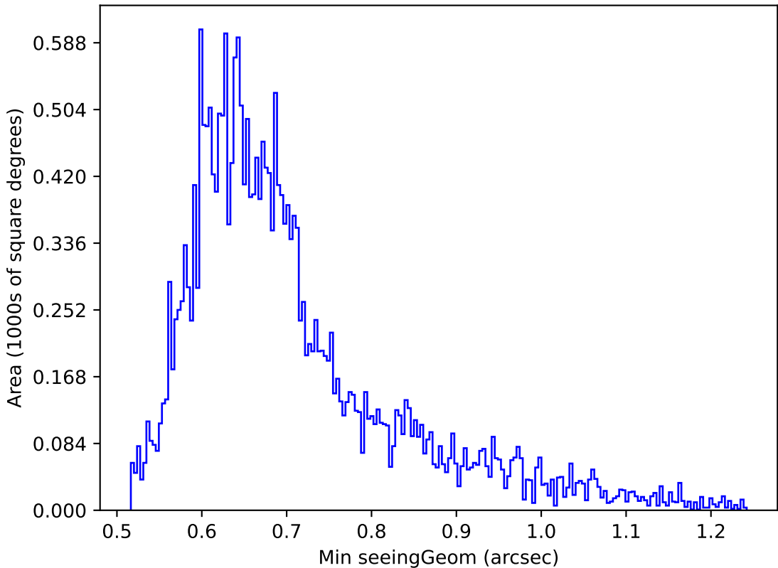
too_elab_r8_d2_giz_v3.4_10yrs Yr 1 g band: Min seeingGeom
