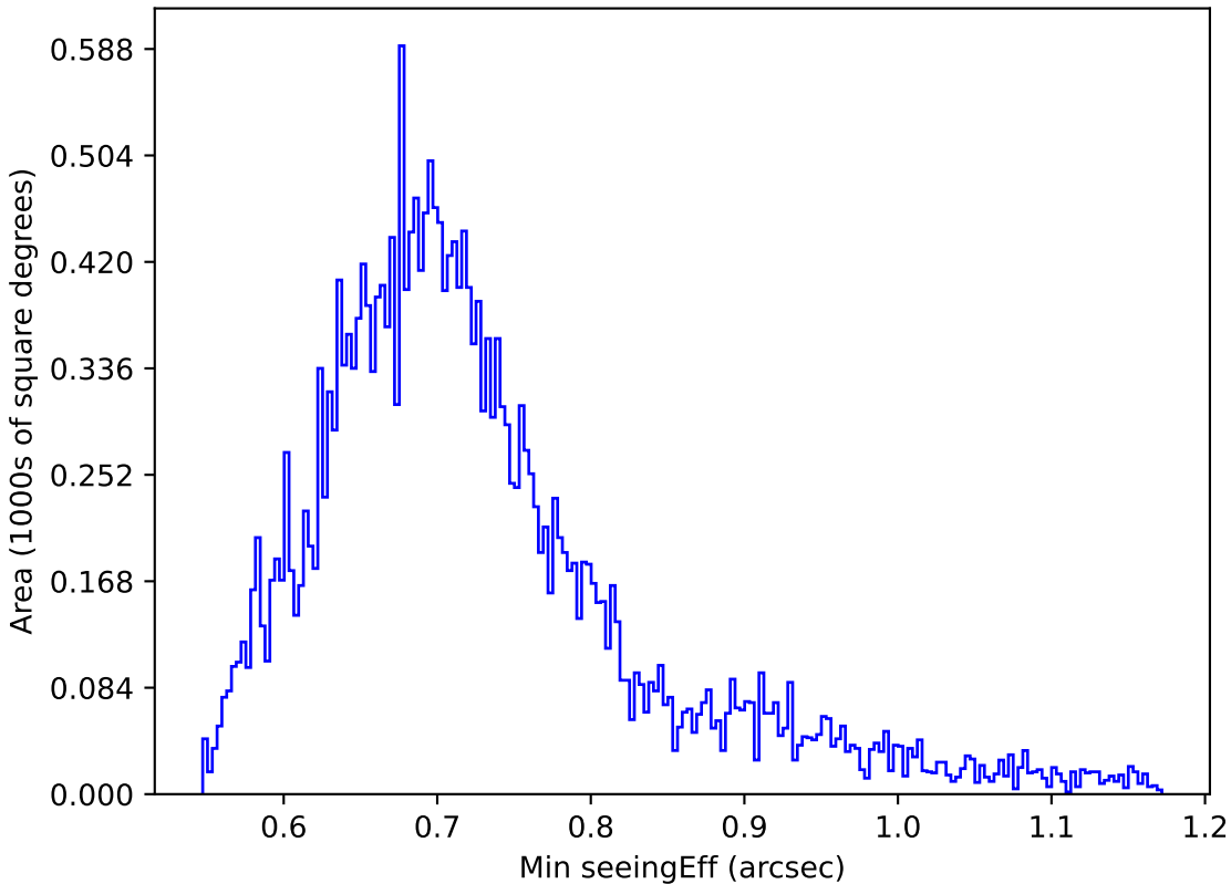
too_elab_r8_d2_giz_v3.4_10yrs Yr 1 z band: Min seeingEff
