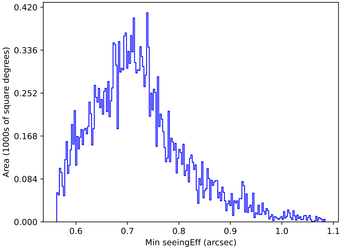
too_elab_r8_d2_giz_v3.4_10yrs Yr 1 y band: Min seeingEff
